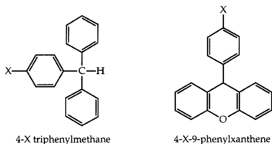
Figure 1. Structures of 4- \chi -triphenylmethane and 4- \chi -9-phenylxanthene
